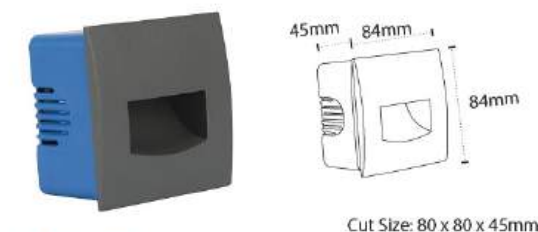
AL 33 - 3W Color Temperature : 3000K, 6000K Material: Die-casting Aluminium, PC Diffuser with ABS Recess Box Body Color: Graphite Gray
