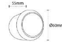
AL 26 B - 3W Color Temperature : 3000K, 6000K Material: Die-casting Aluminium, PC Diffuser with metal recess box Body Color: White
