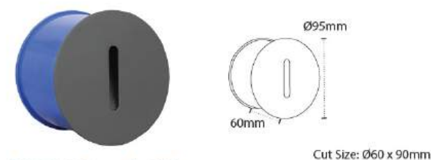
AL 8401 Round - 3W Color Temperature : 3000K, 6000K Material: Die-casting Aluminium, Toughened Glass with ABS Recess Box Body Color: Graphite Gray
