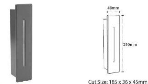
AL 9081 - 3W Color Temperature : 3000K, 6000K Material: Die-casting Aluminium, Toughened Glass with Metal Recess Box Body Color: Graphite Gray
