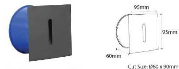
AL 8401 Square - 3W Color Temperature : 3000K, 6000K Material: Die-casting Aluminium, Toughened Glass with ABS Recess Box Body Color: Graphite Gray
